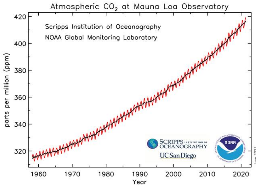
Figure 2: Changes in CO 2 Concentration Over Time (Years)
