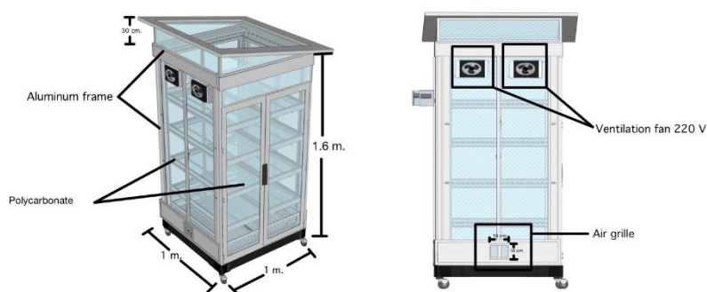
Figure 6-7: Cabinet's draft Figure 8: Shows the pepper drying cabinet, while drying pepper
