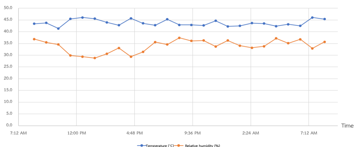
Figure 9: Shows the temperature and relative humidity inside the cabinet.
