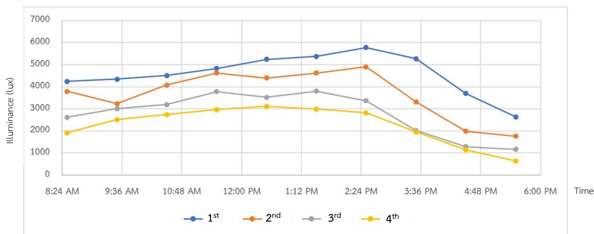
Figure 10: Shows the illuminance inside the cabinet on 1 st - 4 th Layer.
