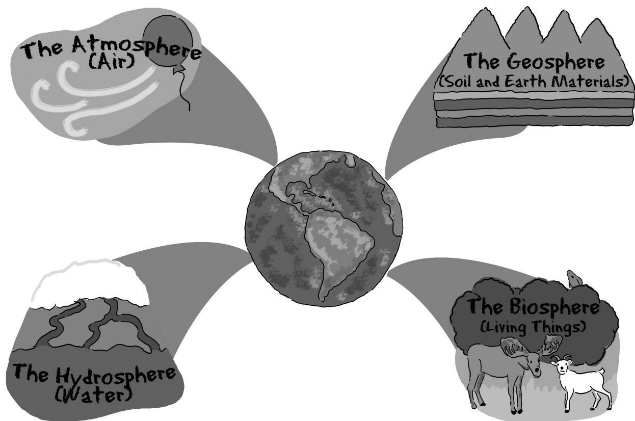
Figure 1: Earth System.
