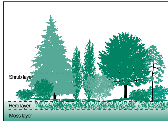
Figure FF-1: Demonstration of a Plant Strata in a Forest Community
