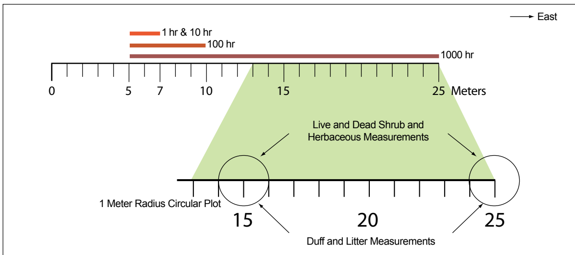
Figure FF-4: Locations of Fuel Measurements along each transect
